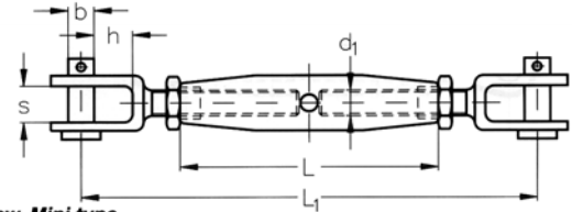
ASS Rigging Screw, Mini type with jaw and jaw
